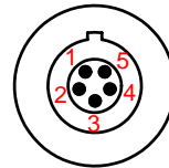
5 PIN MALE BINDER CONNECTOR PINOUT EXT. VIEW
